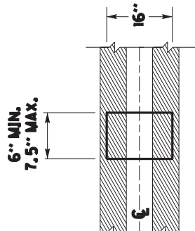
RUMBLE STRIP DETAIL
