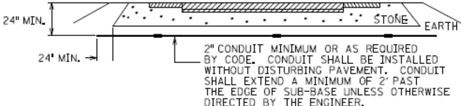
CONDUIT UNDER EXISTING PAVEMENT DETAIL
