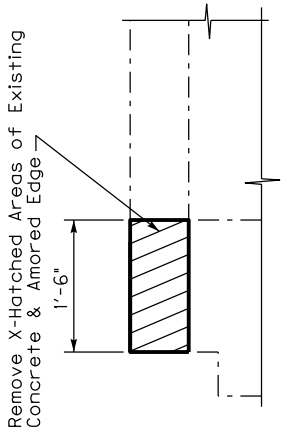
SECTION THROUGH SLAB END Existing
