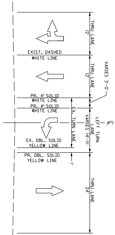
KY 80 OFFSET LEFT TURN LANE STRIPPING TAPER
