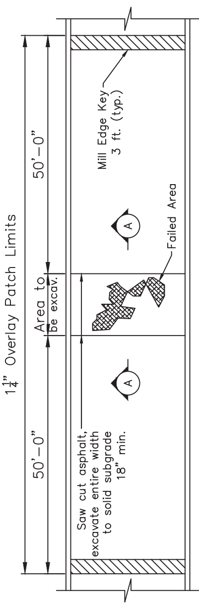
PLAN VIEW
