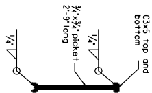
SECTION U-U
