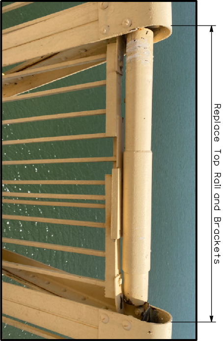
BRIDGE HANDRAIL REPAIRS (Pier 4, Downstream Side)
