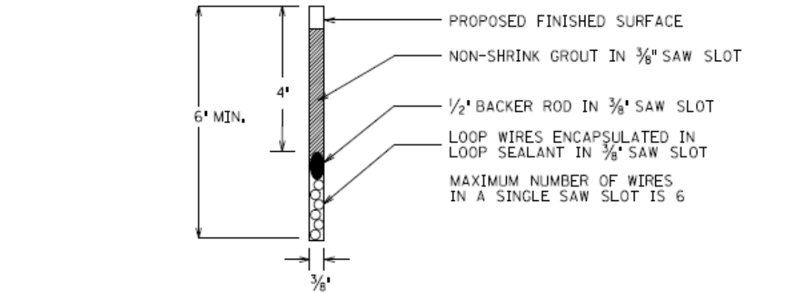
SECTION A-A (SAW SLOT DETAIL)
