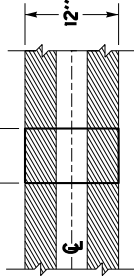
RUMBLE STRIP DETAIL
