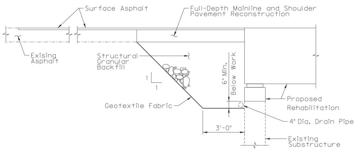
Figure 1: Detail showing proposed work for deck and superstructure replacements
