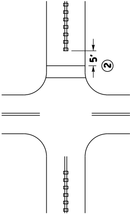
INTERSECTIONS WITHOUT LEFT-TURN LANES ②
