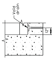
Void Drain Detail
