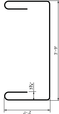
C2(e) Bars #5 Stirrup Bar
