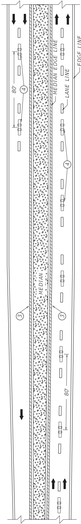
TWO LANE TO FOUR LANE PAVEMENT TRANSITIONS
