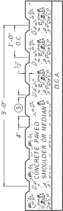
SECTION B-B
