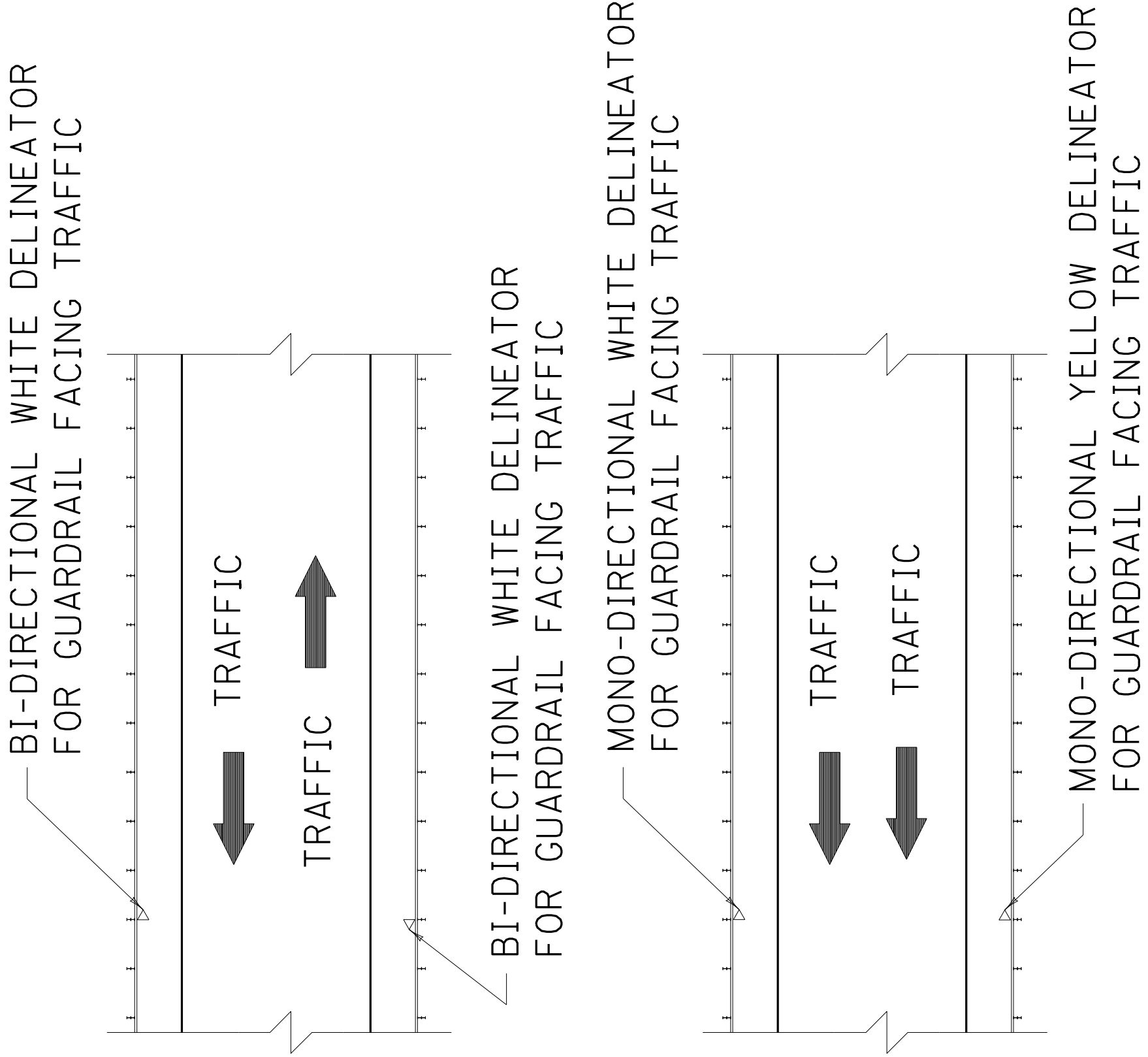
PLACEMENT OF DELINEATORS FOR GUARDRAIL
