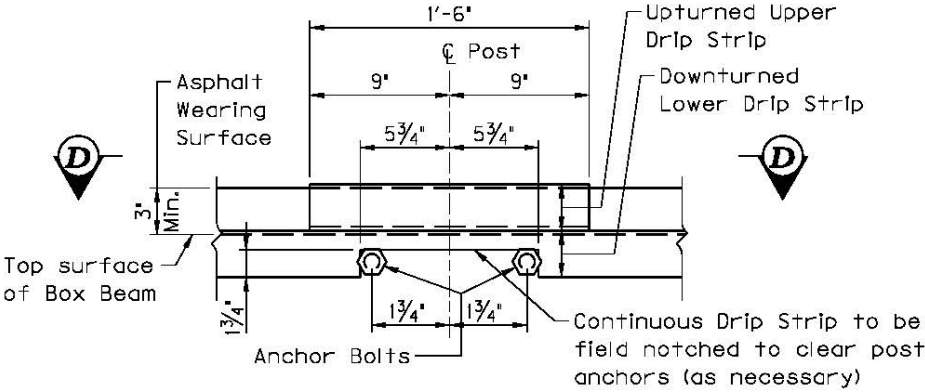
VIEW B-B
