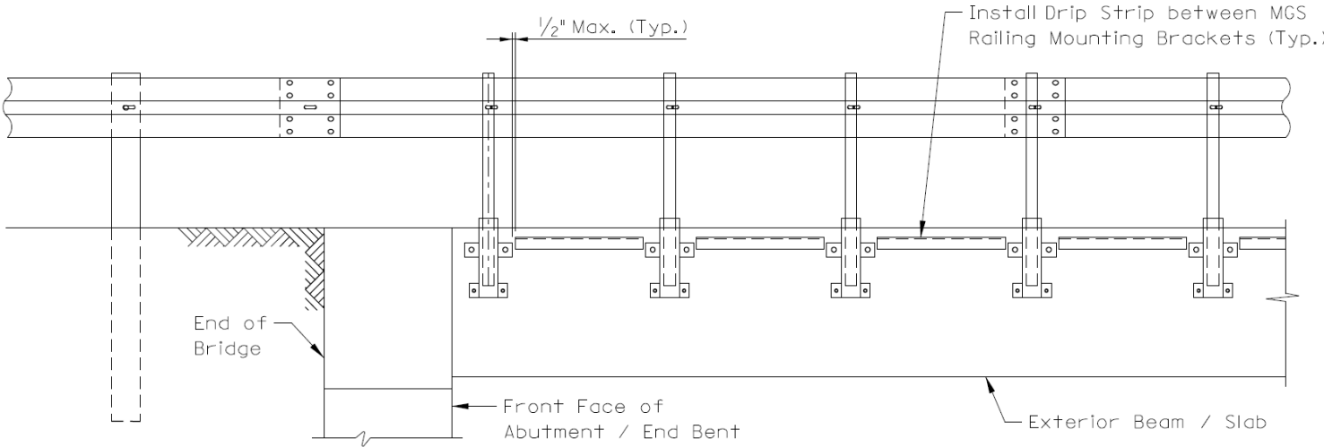
BRIDGE ELEVATION
