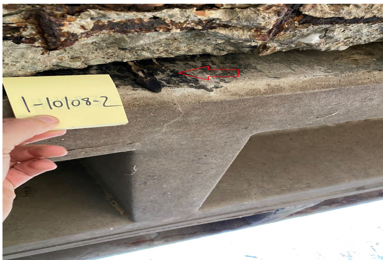
4 - IMG_2696 Joint Between Girders - Facing N - Sample I-10108-2.JPG
