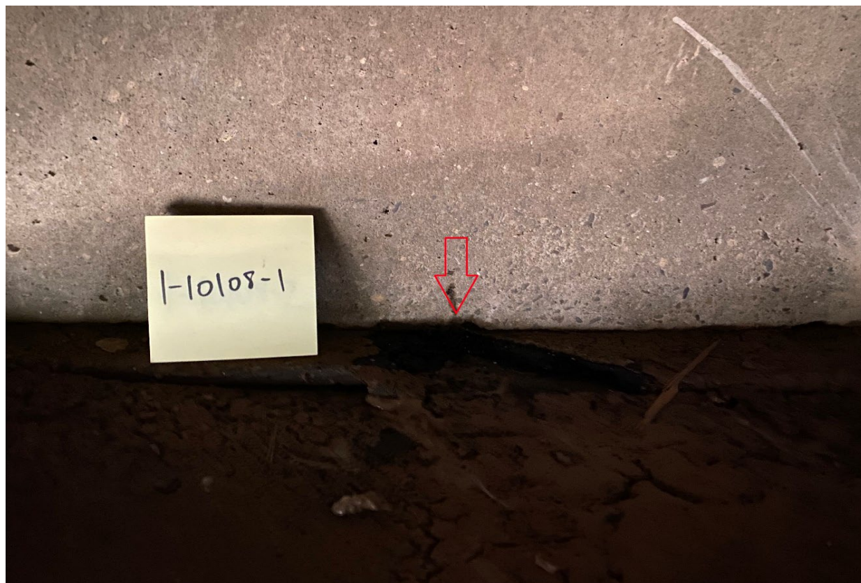
3 - IMG_2695 Abutment Joint - Facing W - Sample I-10108-1.JPG
