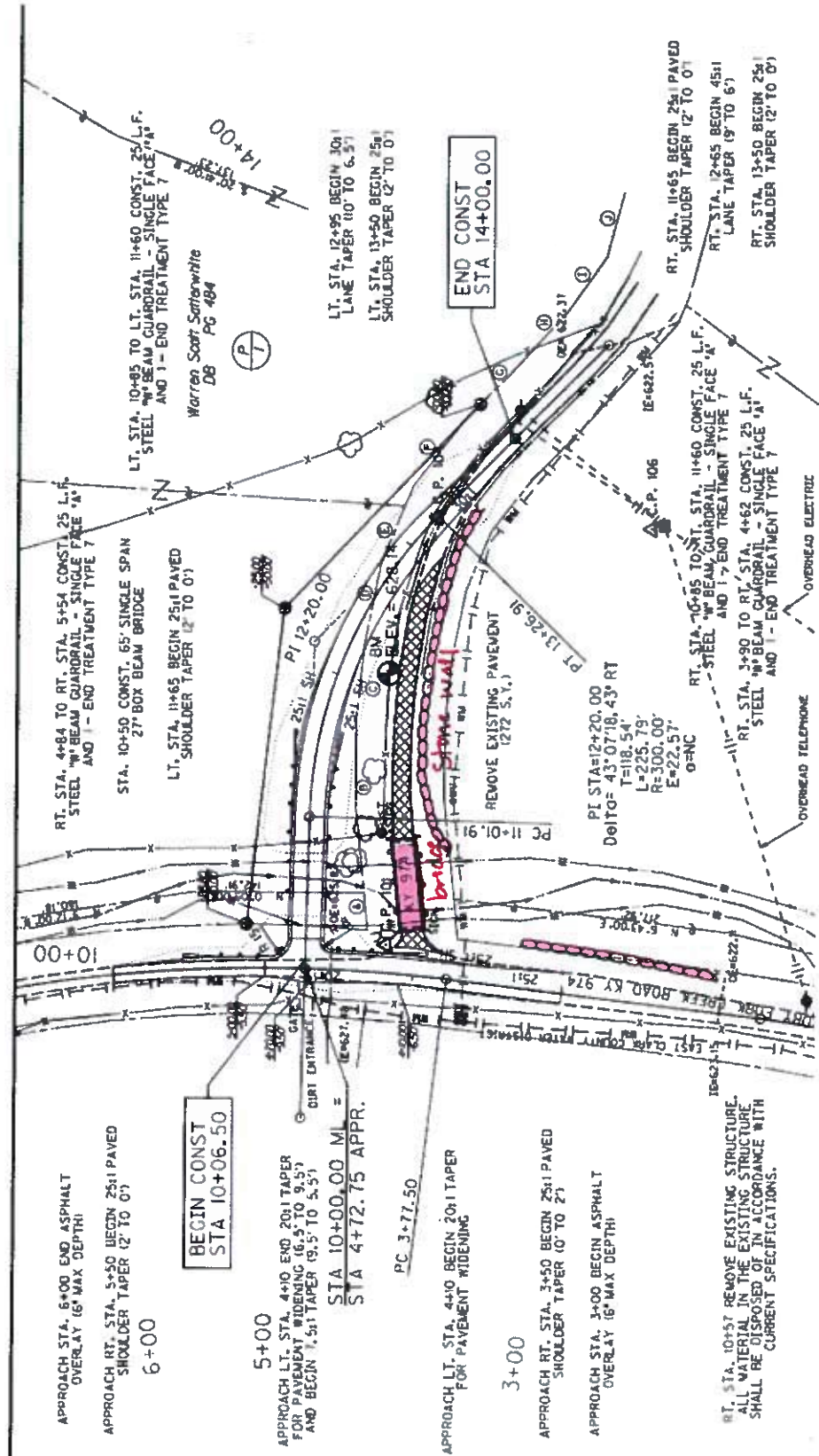
Plan sheet showing stone wall location
