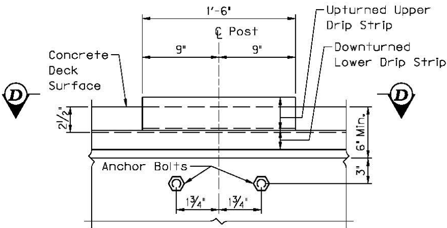
VIEW C-C
