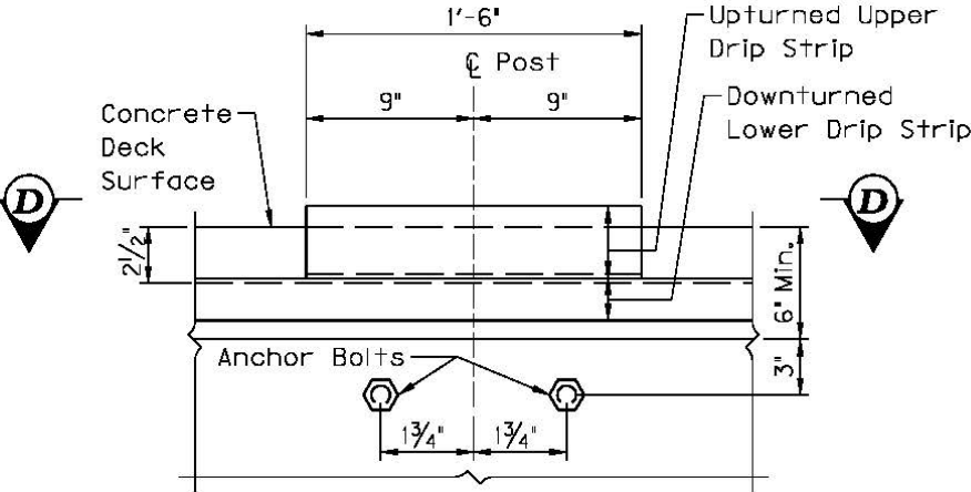
VIEW C-C (Strip shown prior to concrete placement)
