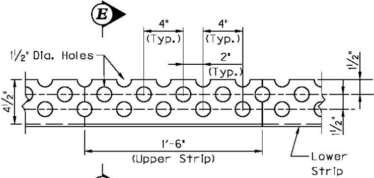
VIEW D-D
