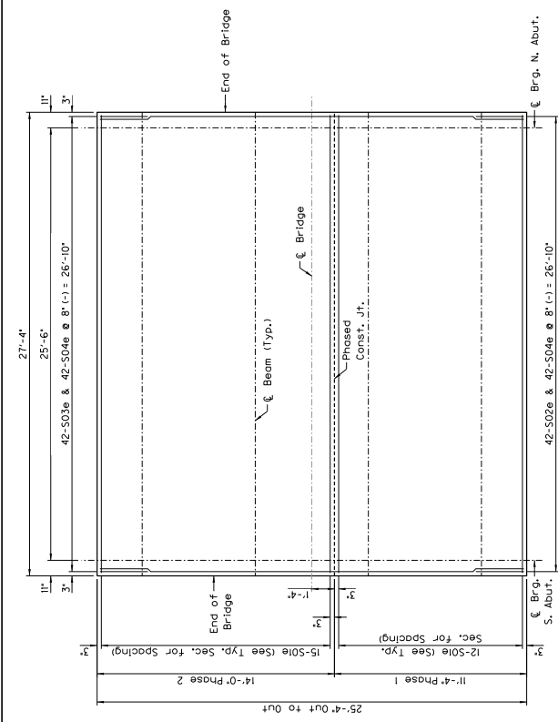
DECK PLAN (Showing Top Rebar)
