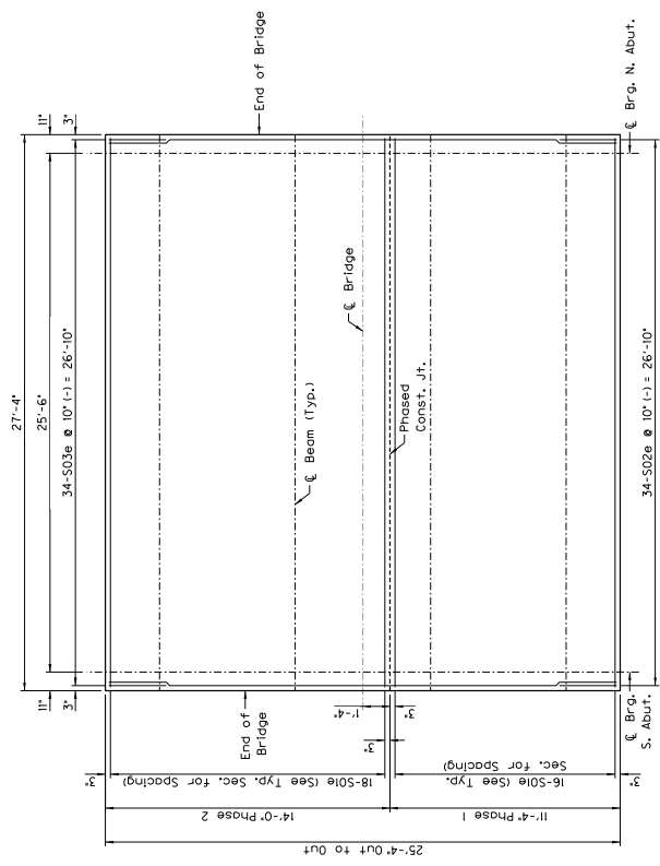
DECK PLAN (Showing Bottom Rebar)
