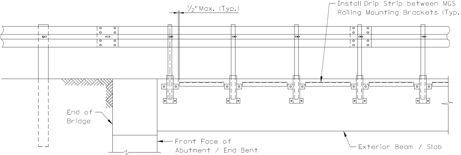
BRIDGE ELEVATION
