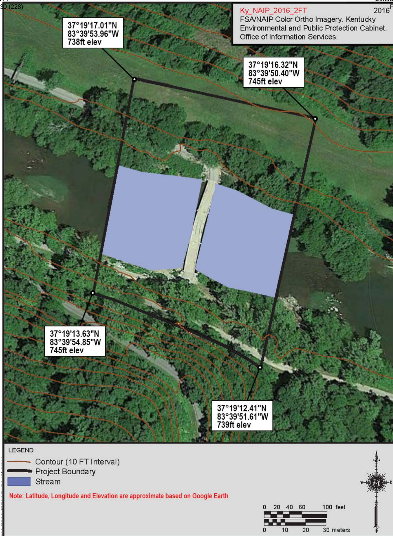
CR 1041 bridge (026C00114N) over South Fork of the Kentucky River (Item No. 11-10082.00) in Clay County, Kentucky.
