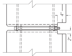
ELEVATION OF CONNECTOR DETAIL
