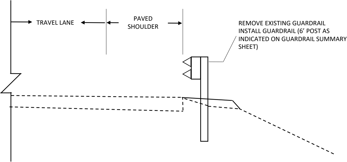
TYPICAL SECTION MP 8.967—11.230
