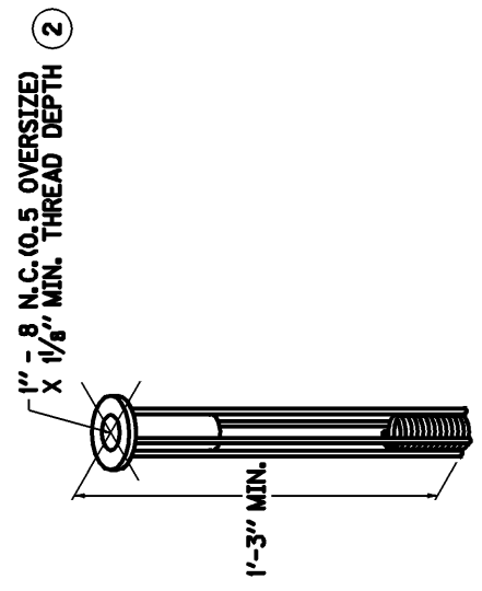
~ ANCHOR PICTORIAL VIEW ~
