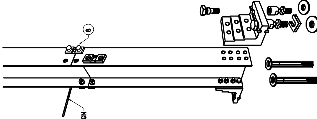
~ PICTORIAL VIEW ~
