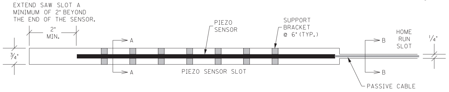
PLAN
