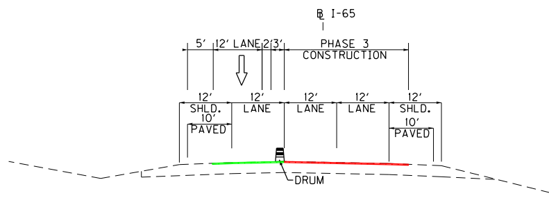
SOUTHBOUND BIFURCATED SECTION
