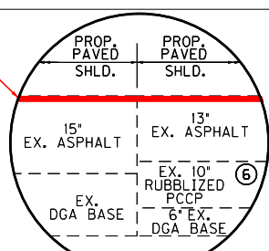
DETAIL "D" NOT TO SCALE
