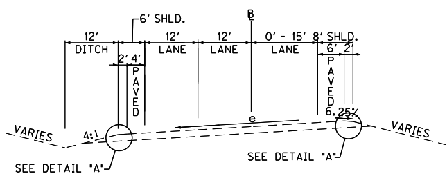
SUPERELEVATED LEFT CUT/FILL SECTION
