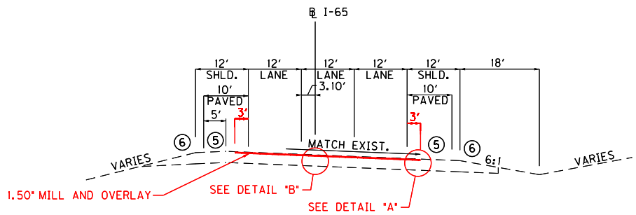
SUPERELEVATED LEFT NORTHBOUND BIFURCATED FILL/CUT SECTION
