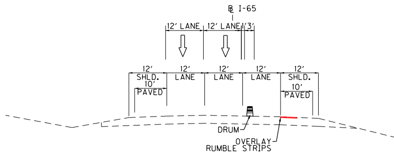
SOUTHBOUND BIFURCATED SECTION
