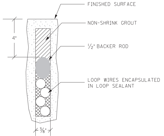
SECTION A-A (ASPHALT)
