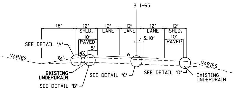
LEFT SUPERELEVATED SOUTHBOUND BIFURCATED CUT/FILL SECTION
