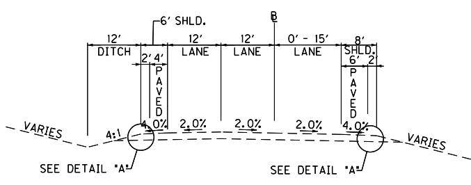
NORMAL CUT/FILL SECTION
