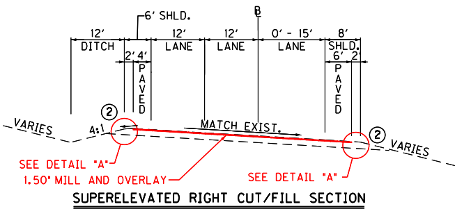
SUPERELEVATED RIGHT CUT/FILL SECTION
