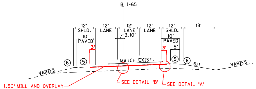
SUPERELEVATED RIGHT NORTHBOUND BIFURCATED FILL/CUT SECTION
