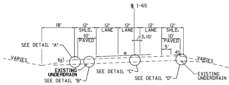
RIGHT SUPERELEVATED SOUTHBOUND BIFURCATED CUT/FILL SECTION
