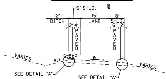
SUPERELEVATED RIGHT CUT/FILL SECTION
