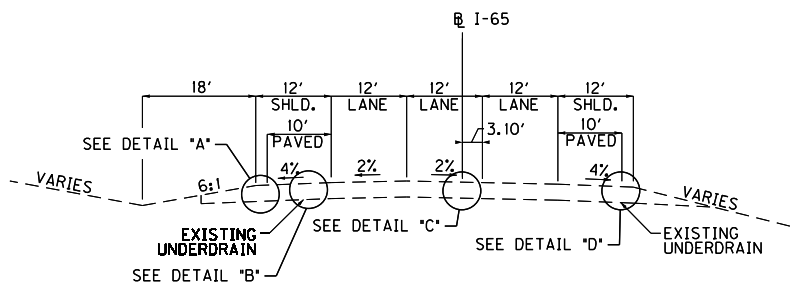
NORMAL SOUTHBOUND BIFURCATED CUT/FILL SECTION
