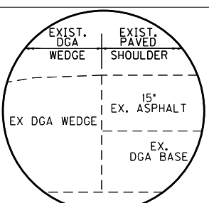
DETAIL "F" NOT TO SCALE
