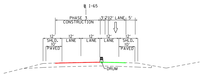
NORTHBOUND BIFURCATED SECTION
