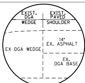
DETAIL "H" NOT TO SCALE
