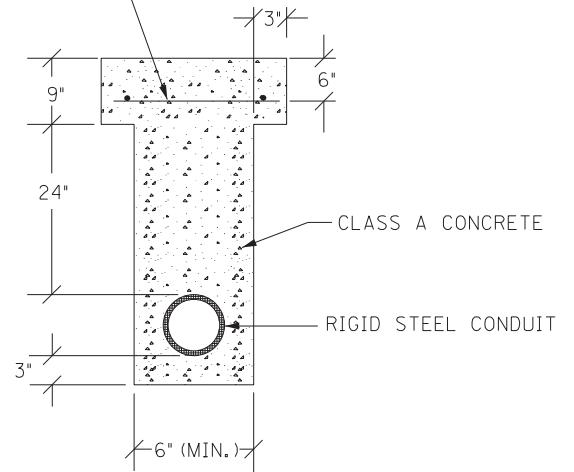
OPEN CUT PAVEMENT DETAIL
