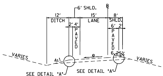
SUPERELEVATED LEFT CUT/FILL SECTION
