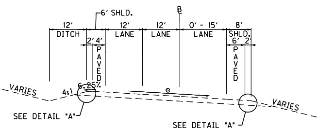
SUPERELEVATED RIGHT CUT/FILL SECTION
