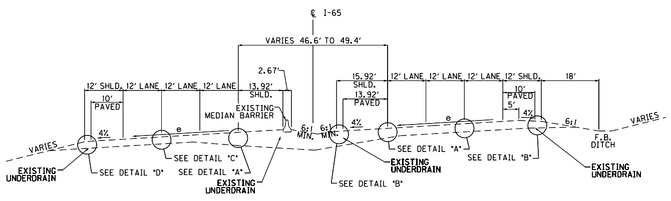
SUPERELEVATED BARRIER TRANSITION FILL/CUT SECTION
