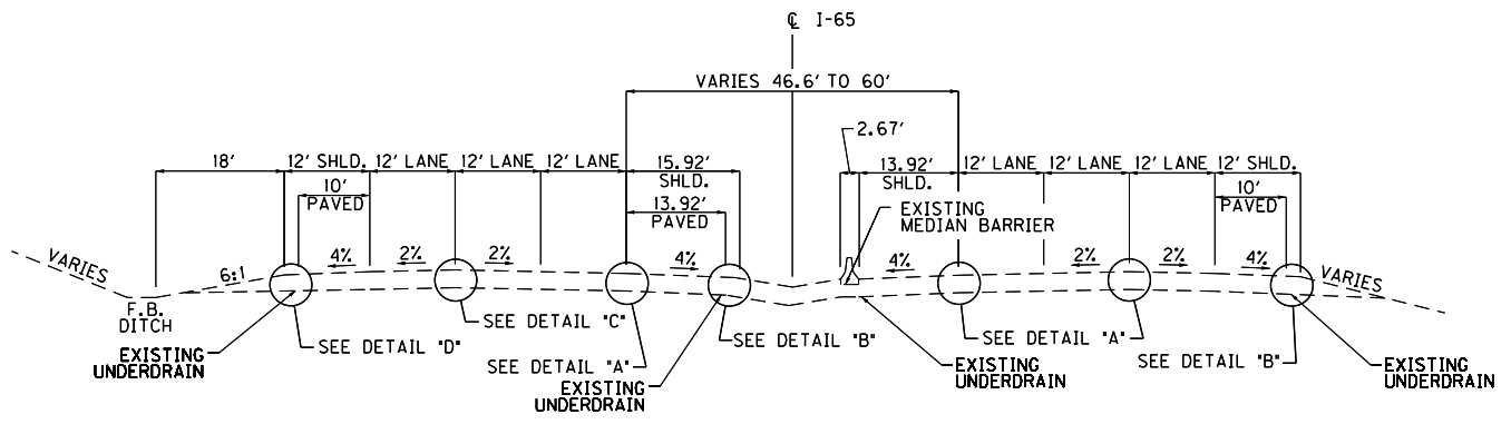
NORMAL BARRIER TRANSITION CUT/FILL SECTION
