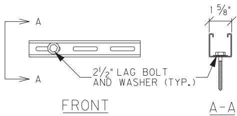
METAL FRAMING CHANNEL
