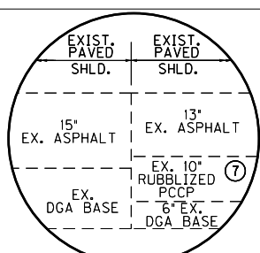
DETAIL "E" NOT TO SCALE
