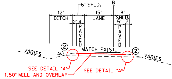
NORMAL CUT/FILL SECTION
