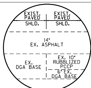
DETAIL "G" NOT TO SCALE
