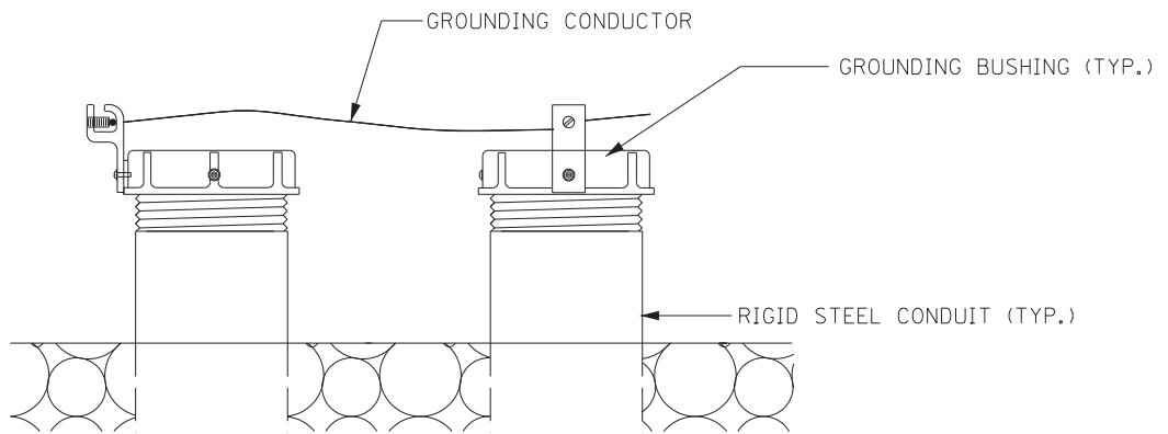
GROUNDING DETAIL
