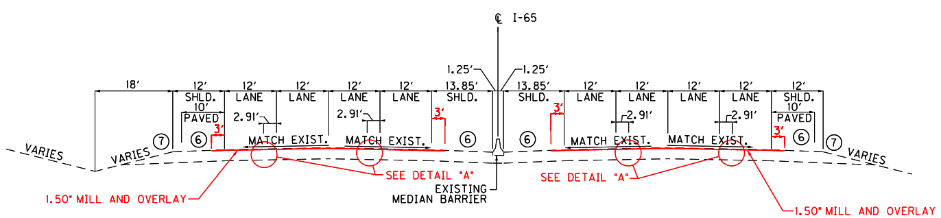
NORMAL EIGHT LANE CUT/FILL SECTION
