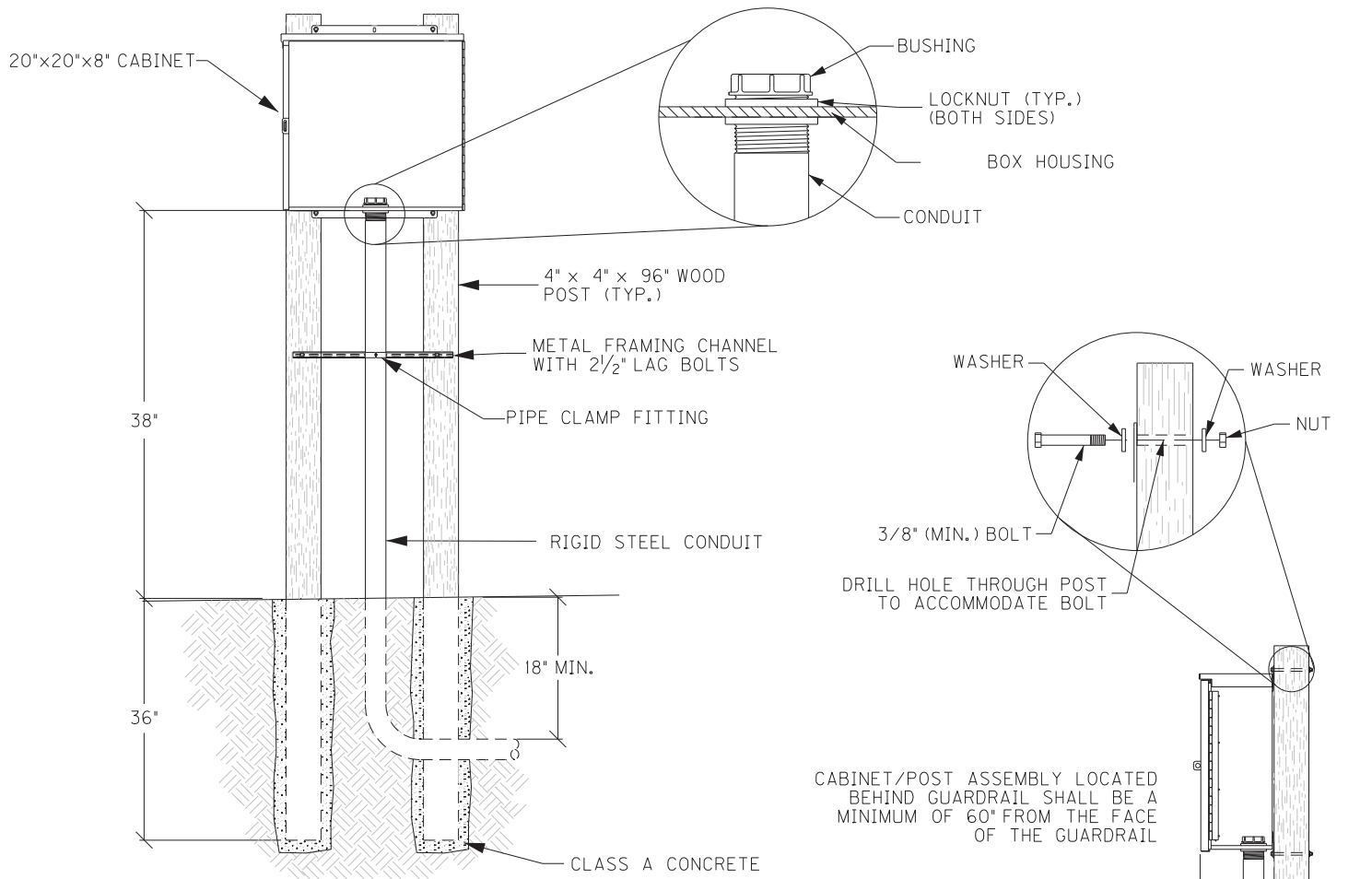
FRONT VIEW
