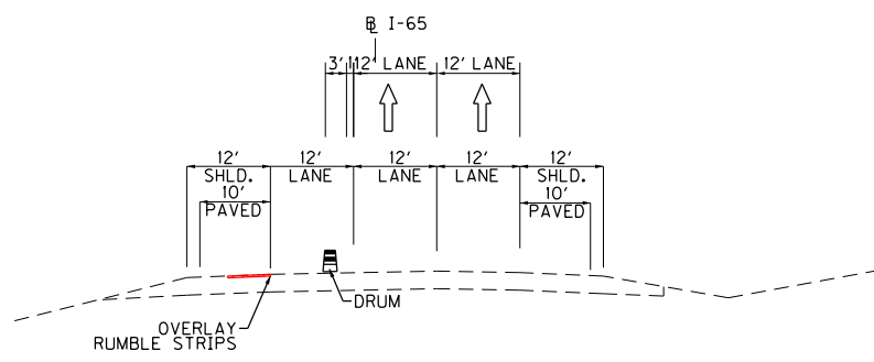
NORTHBOUND BIFURCATED SECTION
