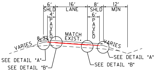
US 41A RAMP RIGHT SUPERELEVATED SECTION
