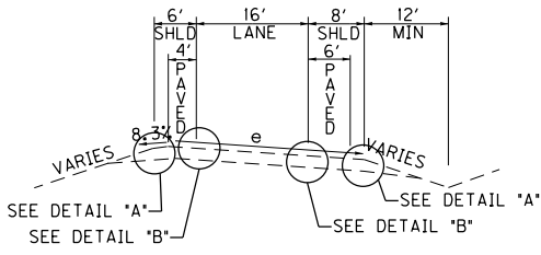
US 41A RAMP RIGHT SUPERELEVATED SECTION
