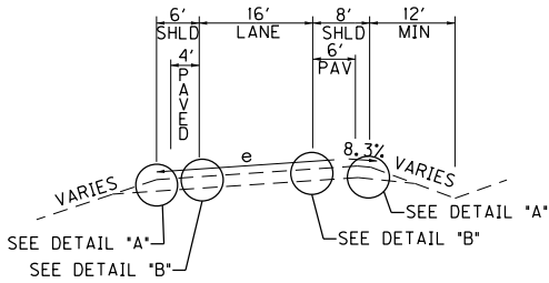
US 41A RAMP LEFT SUPERELEVATED SECTION
