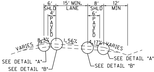
US 41A RAMP NORMAL SECTION
