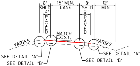
US 41A RAMP NORMAL SECTION
