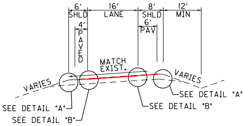
US 41A RAMP LEFT SUPERELEVATED SECTION
