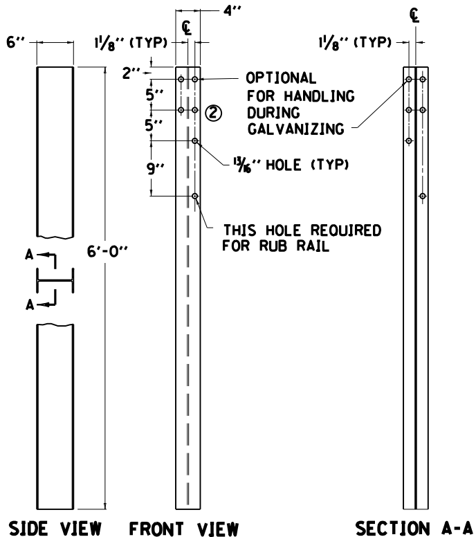
~ W6 X 9.0 STEEL POST ① ~
