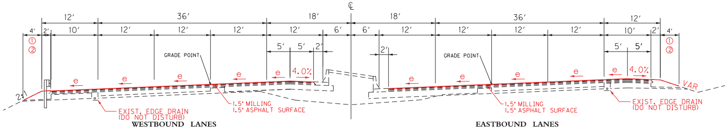
SUPERELEVATED SECTION
