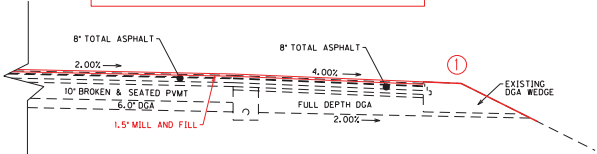
DETAIL 'A-C' NORMAL SECTION
