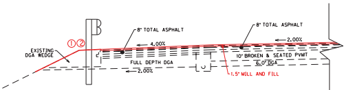
DETAIL 'A-A' NORMAL SECTION
