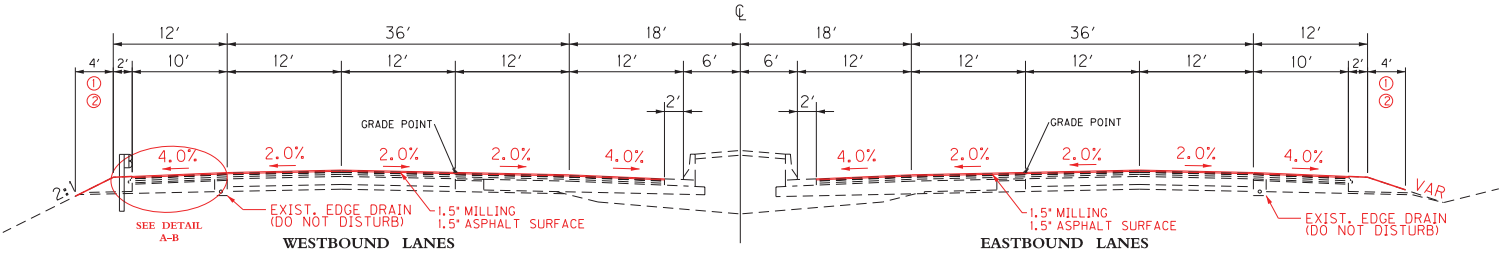
NORMAL SECTION
