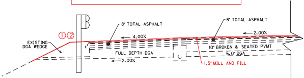
DETAIL 'A-B' NORMAL SECTION
