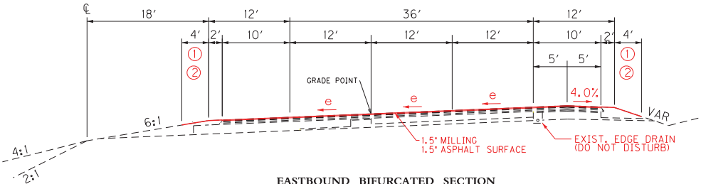
EASTBOUND BIFURCATED SECTION SUPERELEVATED SECTION
