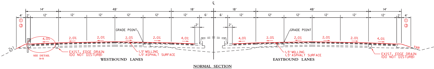
NORMAL SECTION
