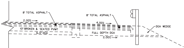
DETAIL 'A'
