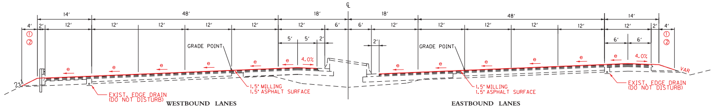
SUPERELEVATED SECTION
