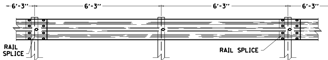
ELEVATION VIEW
