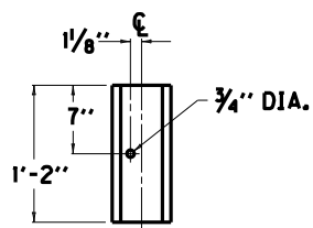
REAR ELEVATION
