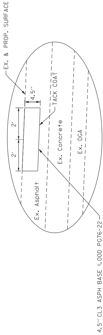
DETAIL A
