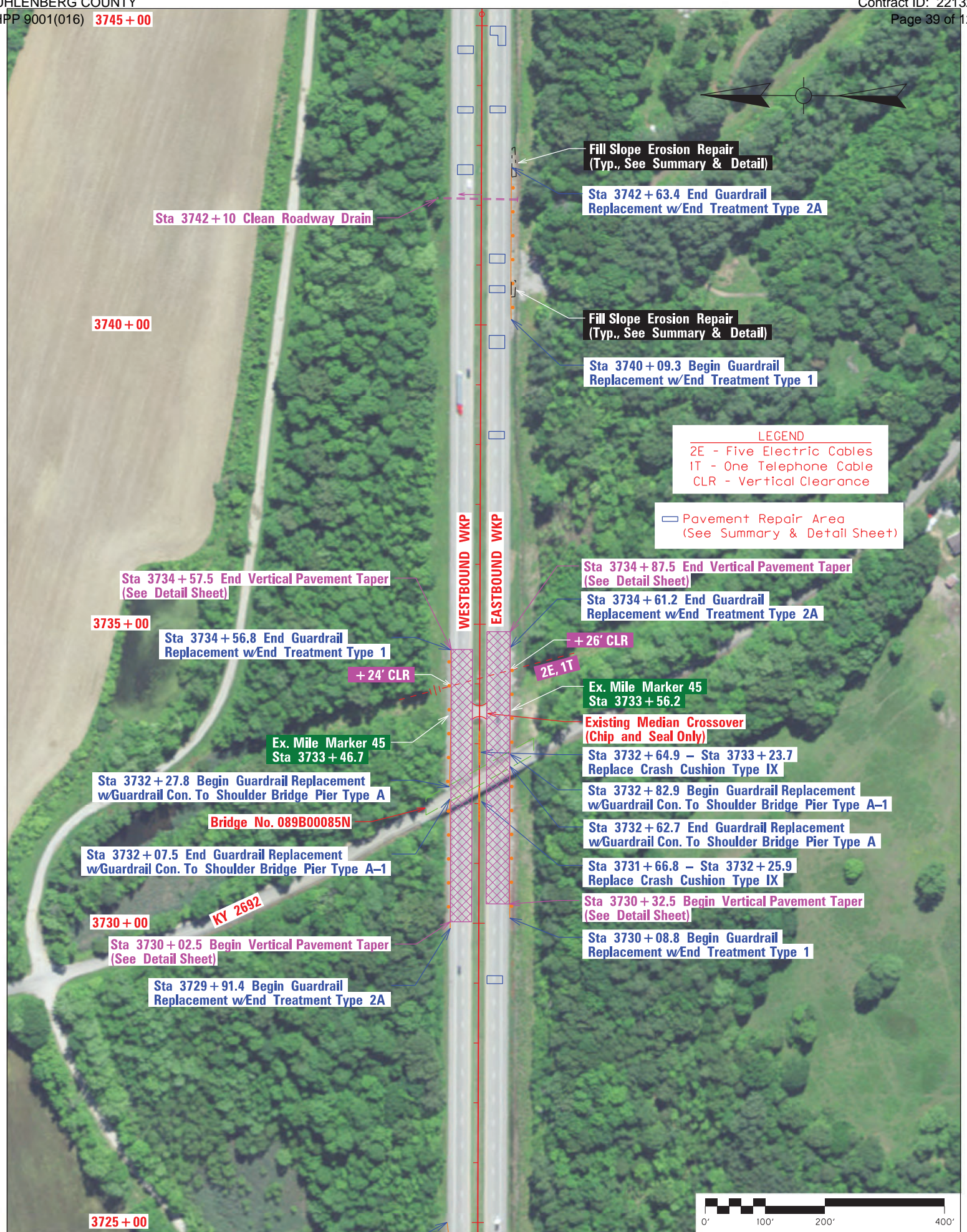
WKP Rehab Plan - Scale 1" = 200' - Sheet 5 of 7 - Sta 3725+00 to Sta 3745+00
