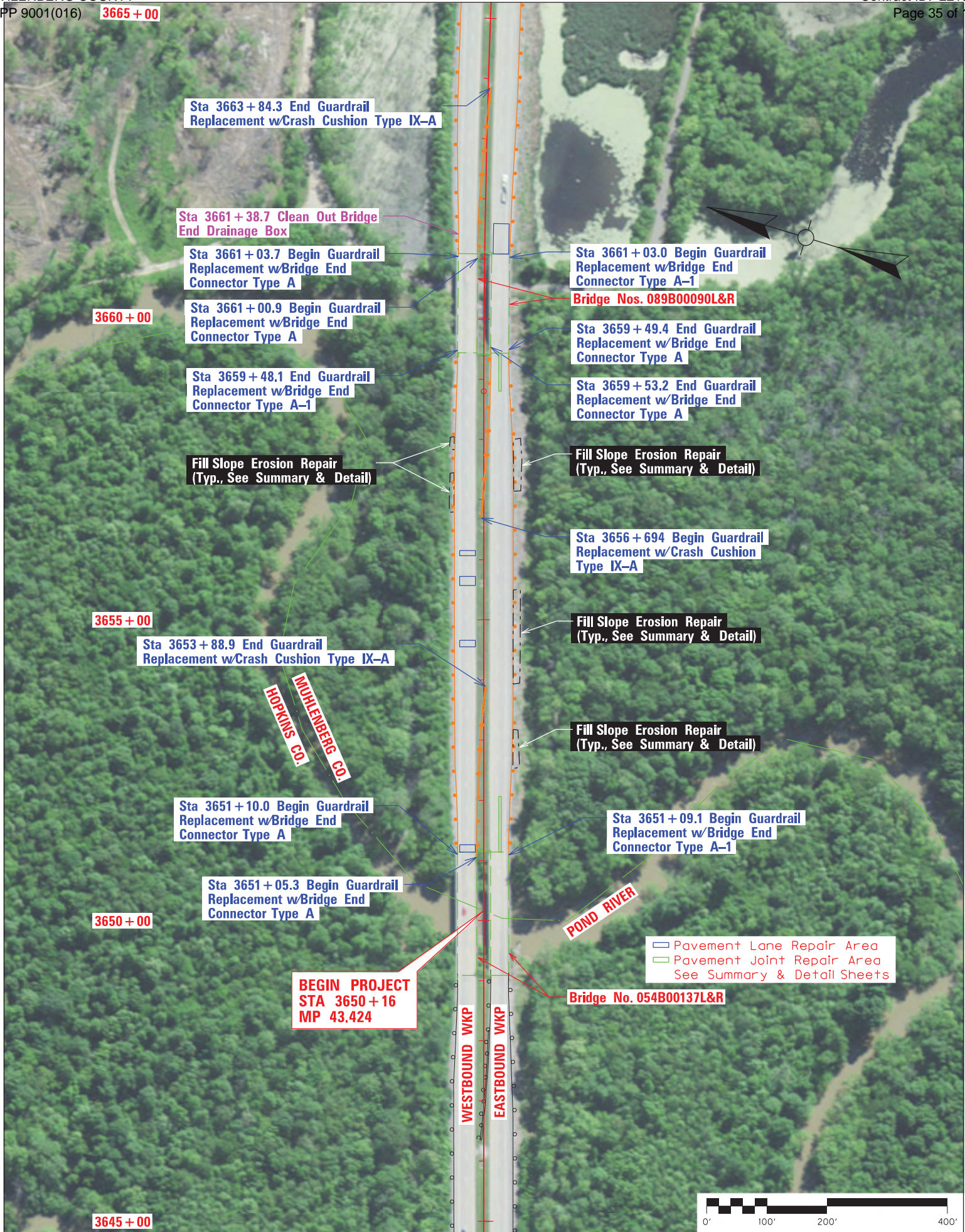
WKP Rehab Plan - Scale 1" = 200' - Sheet 1 of 7 - Sta 3645+00 to Sta 3665+00
