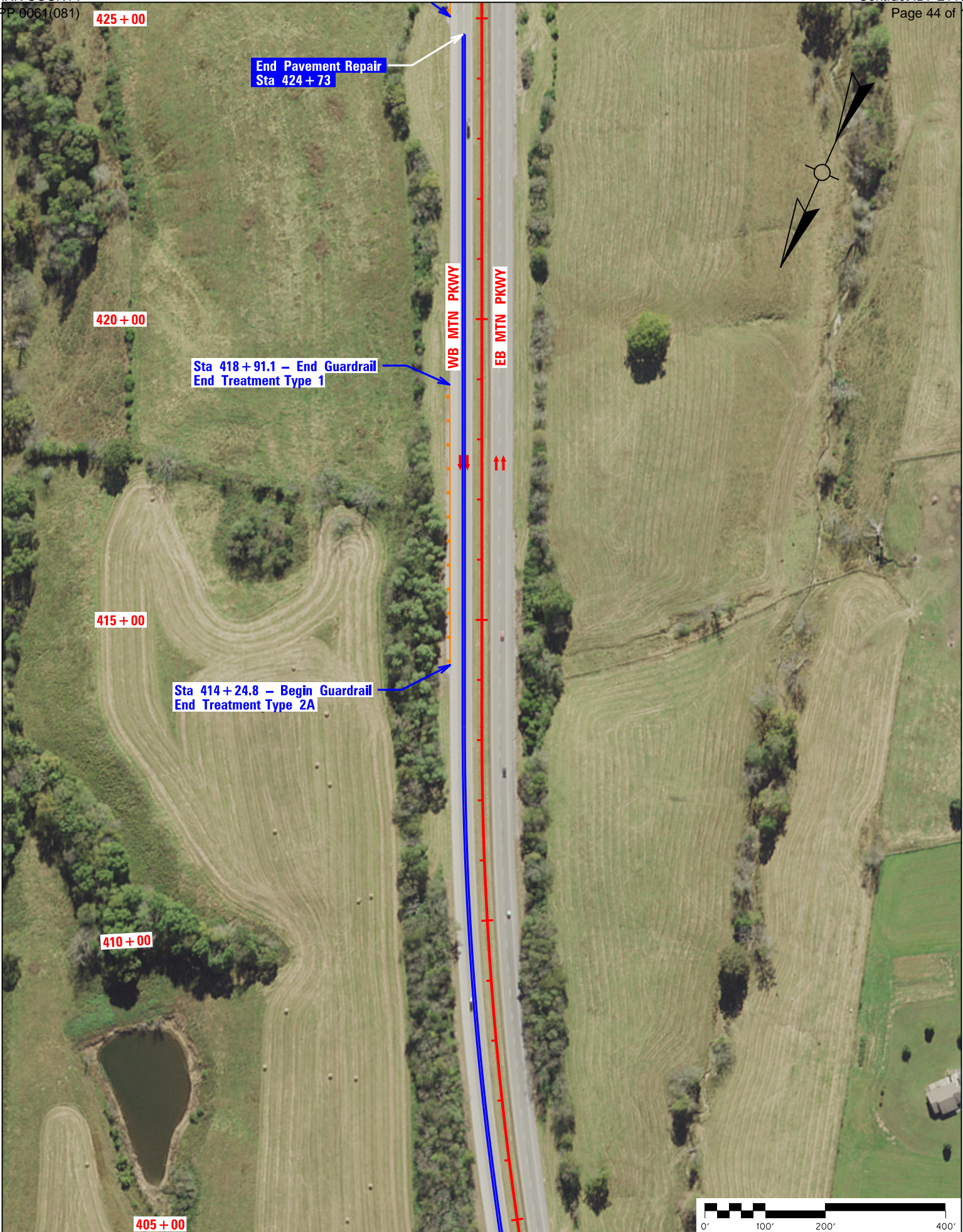
Mountain Parkway Rehab Plan - Scale 1" = 200' - Sheet 7 of 18 - Sta 405+00 to Sta 425+00
