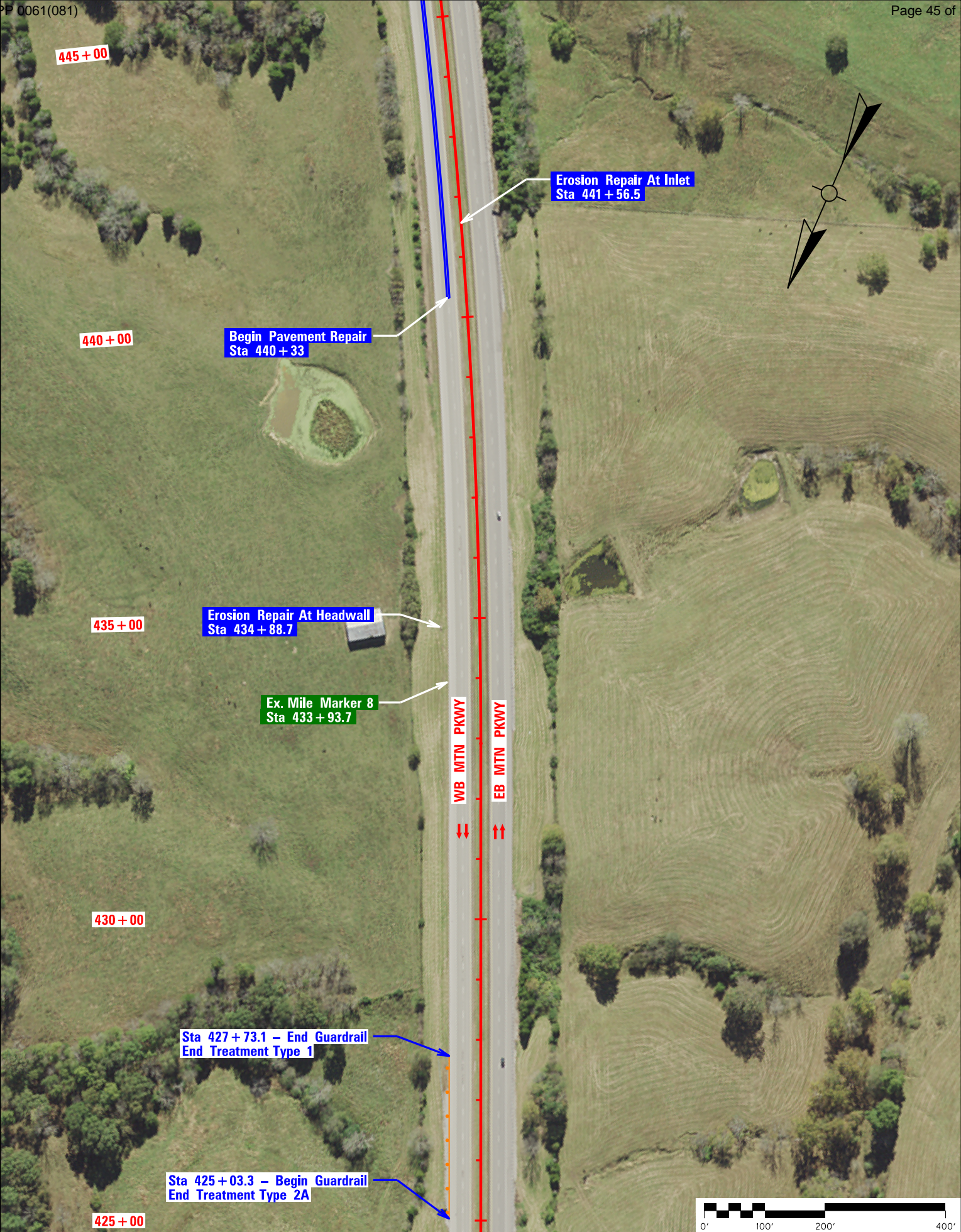
Mountain Parkway Rehab Plan - Scale 1" = 200' - Sheet 8 of 18 - Sta 425+00 to Sta 445+00
