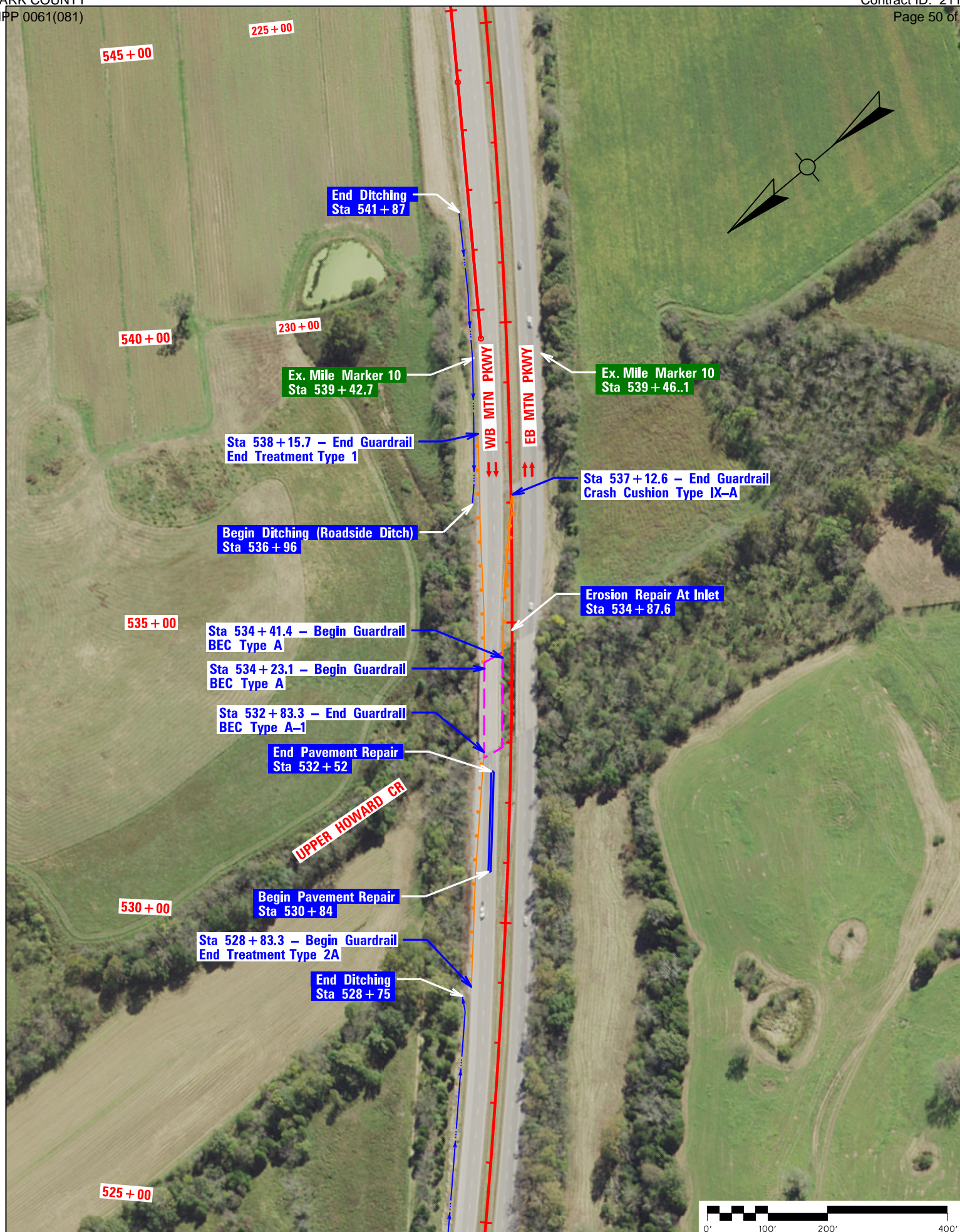
Mountain Parkway Rehab Plan - Scale 1" = 200' - Sheet 13 of 18 - Sta 525+00 to Sta 545+00
