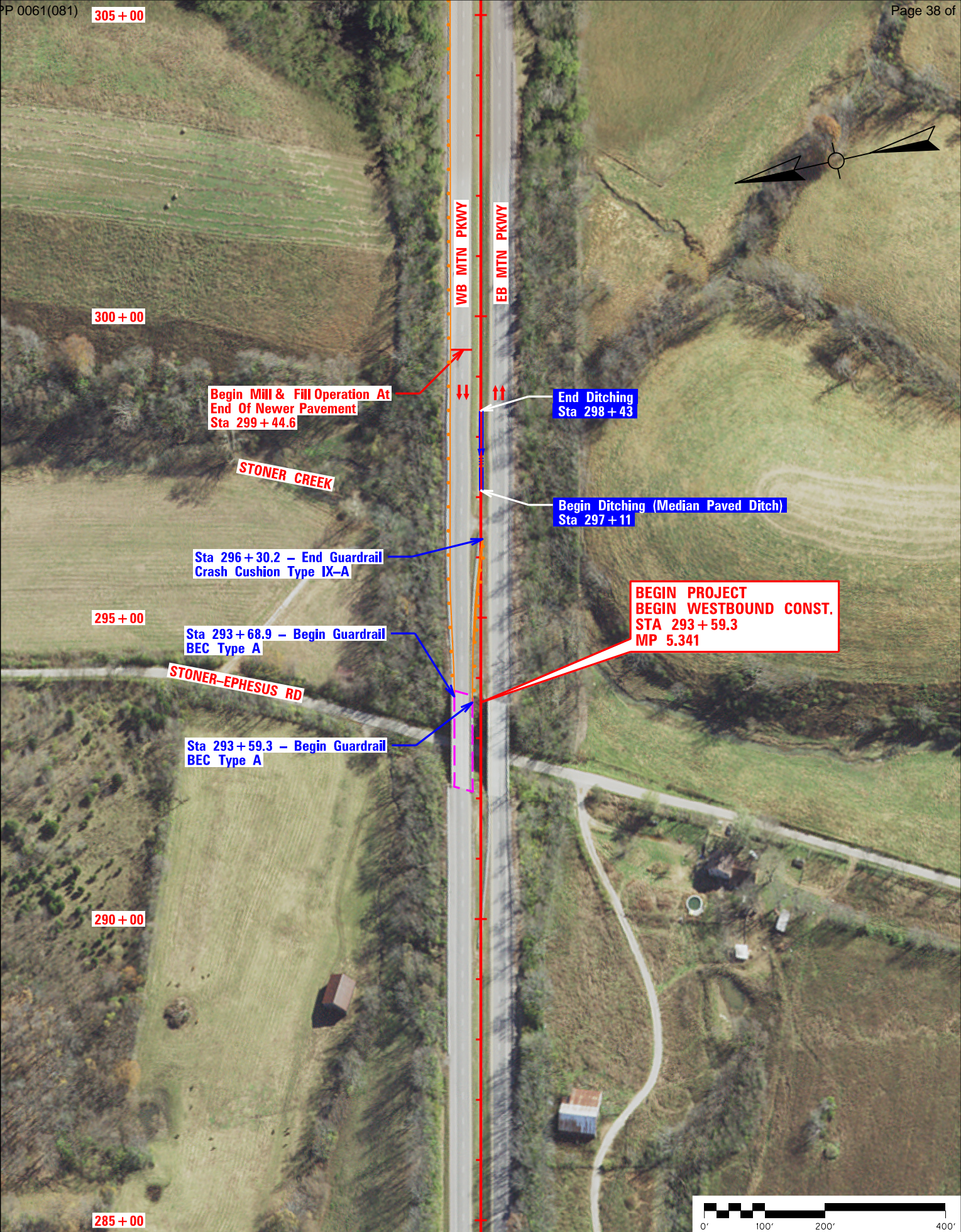
Mountain Parkway Rehab Plan - Scale 1" = 200' - Sheet 1 of 18 - Sta 285+00 to Sta 305+00
