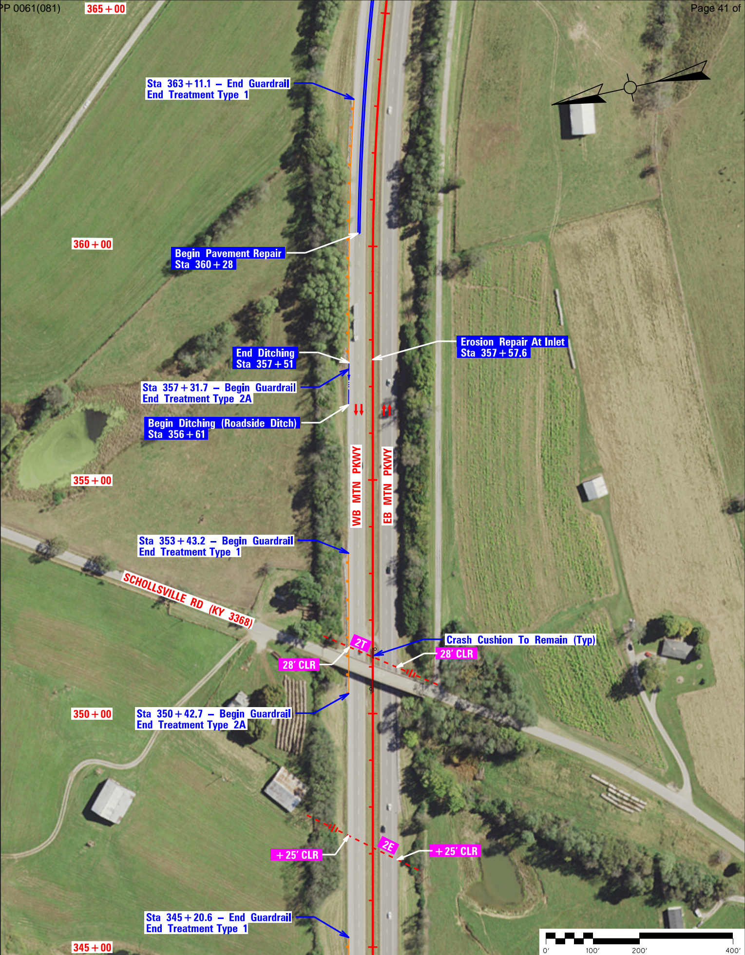
Mountain Parkway Rehab Plan - Scale 1" = 200' - Sheet 4 of 18 - Sta 345+00 to Sta 365+00
