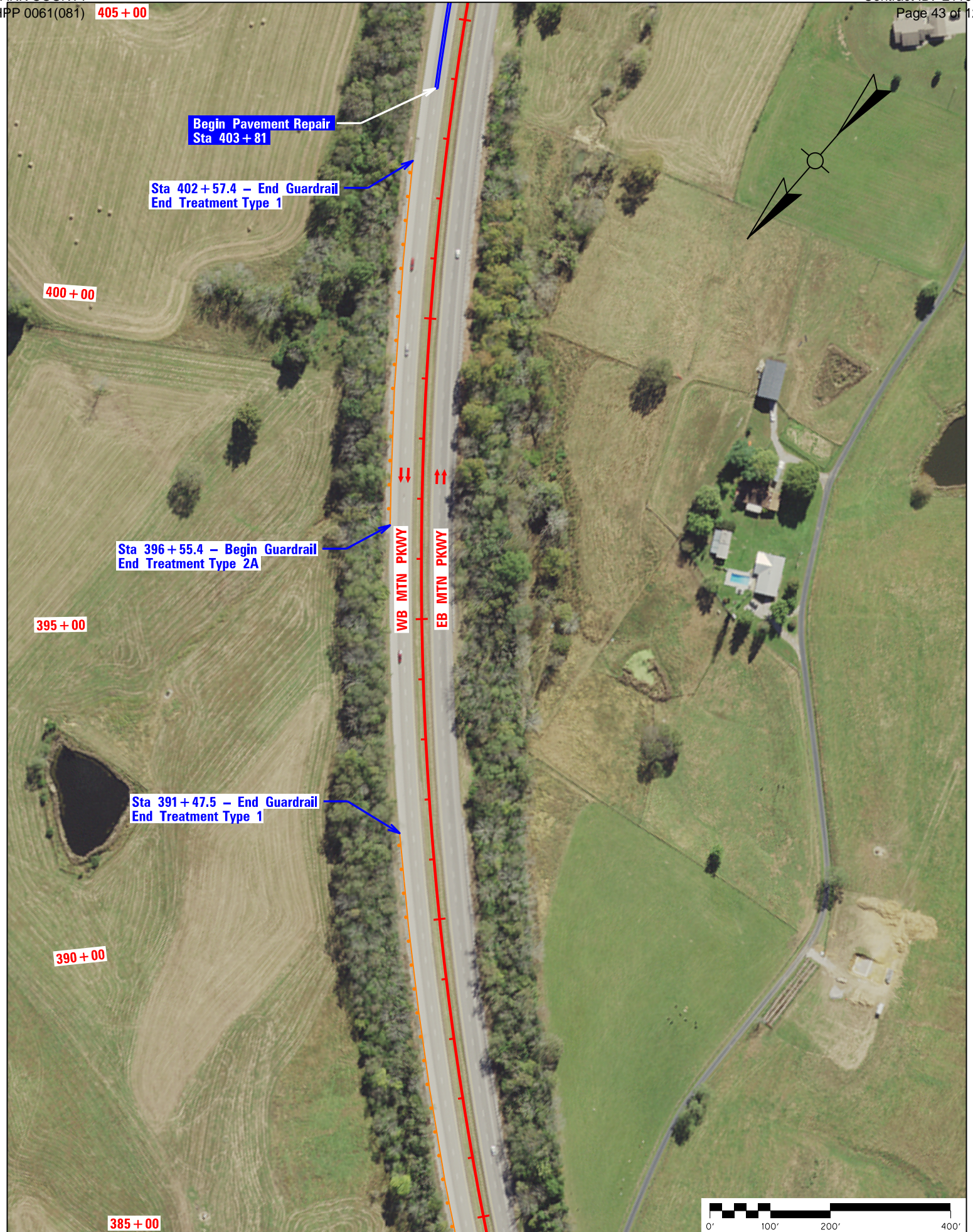
Mountain Parkway Rehab Plan - Scale 1" = 200' - Sheet 6 of 18 - Sta 385+00 to Sta 405+00
