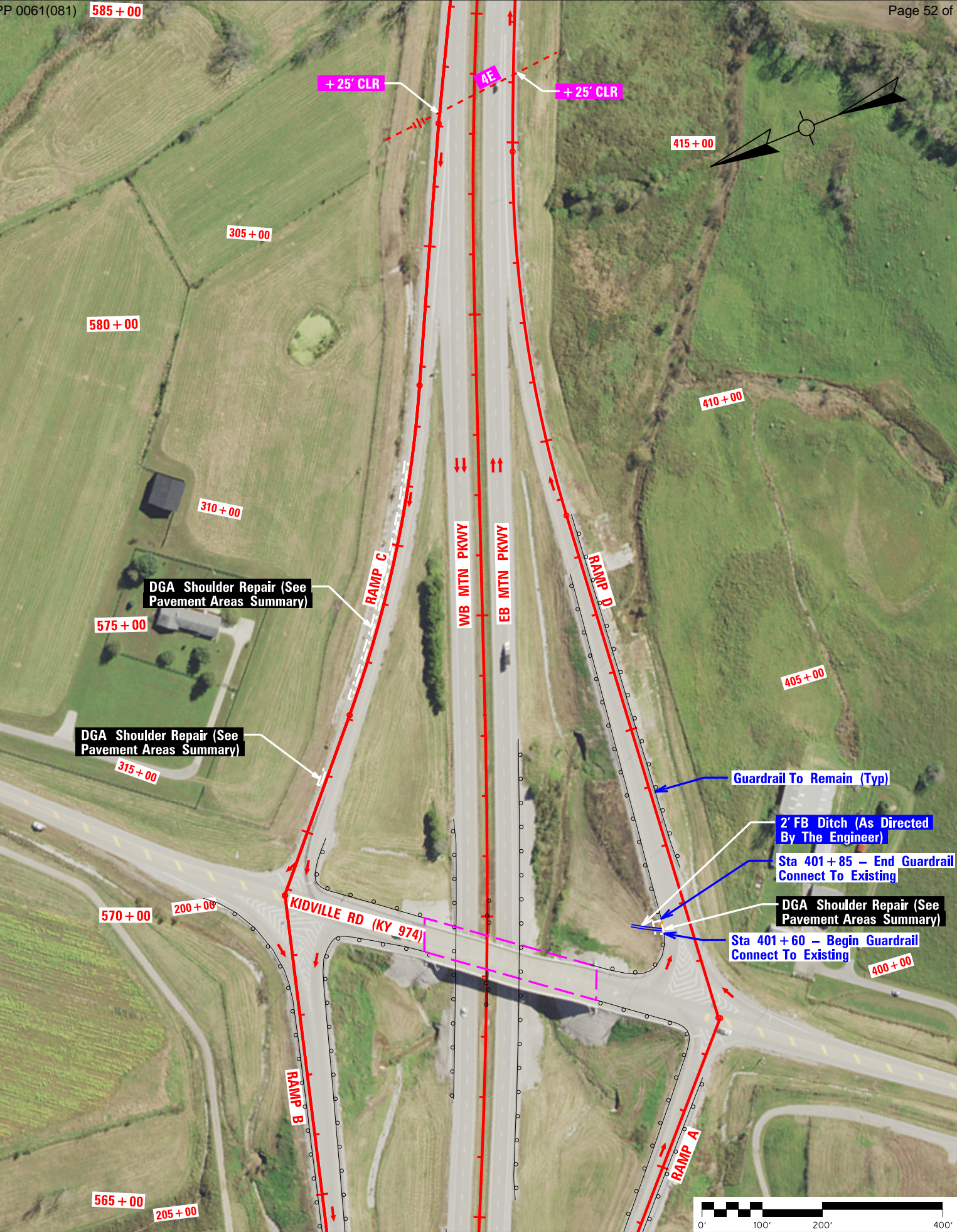
Mountain Parkway Rehab Plan - Scale 1" = 200' - Sheet 15 of 18 - Sta 565+00 to Sta 585+00
