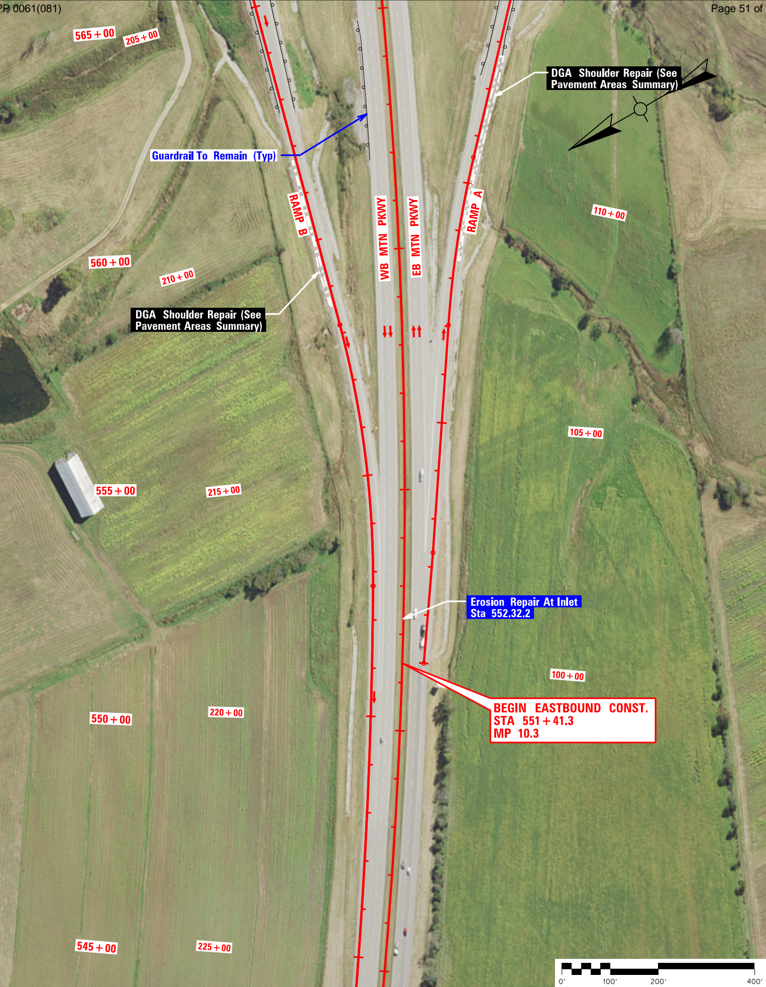
Mountain Parkway Rehab Plan - Scale 1" = 200' - Sheet 14 of 18 - Sta 545+00 to Sta 565+00
