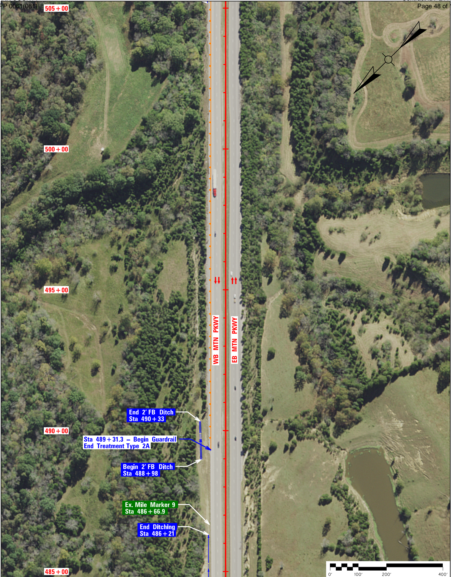
Mountain Parkway Rehab Plan - Scale 1" = 200' - Sheet II of 18 - Sta 485+00 to Sta 505+00
