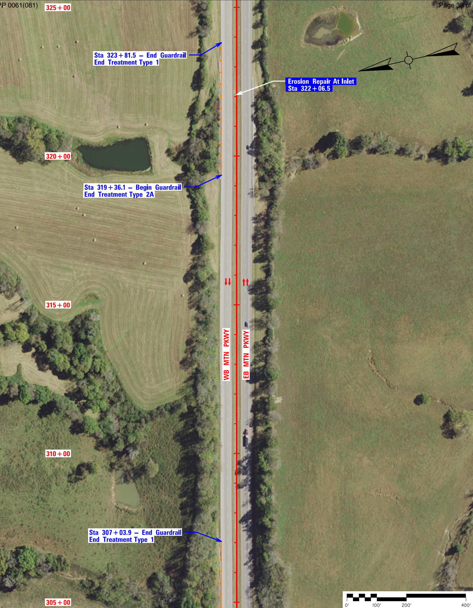
Mountain Parkway Rehab Plan - Scale 1" = 200' - Sheet 2 of 18 - Sta 305+00 to Sta 325+00
