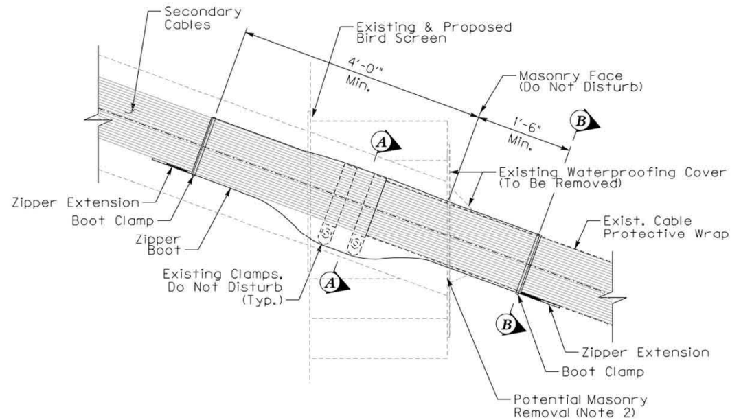
TYPICAL SECONDARY CABLE LOCATION ELEVATION
