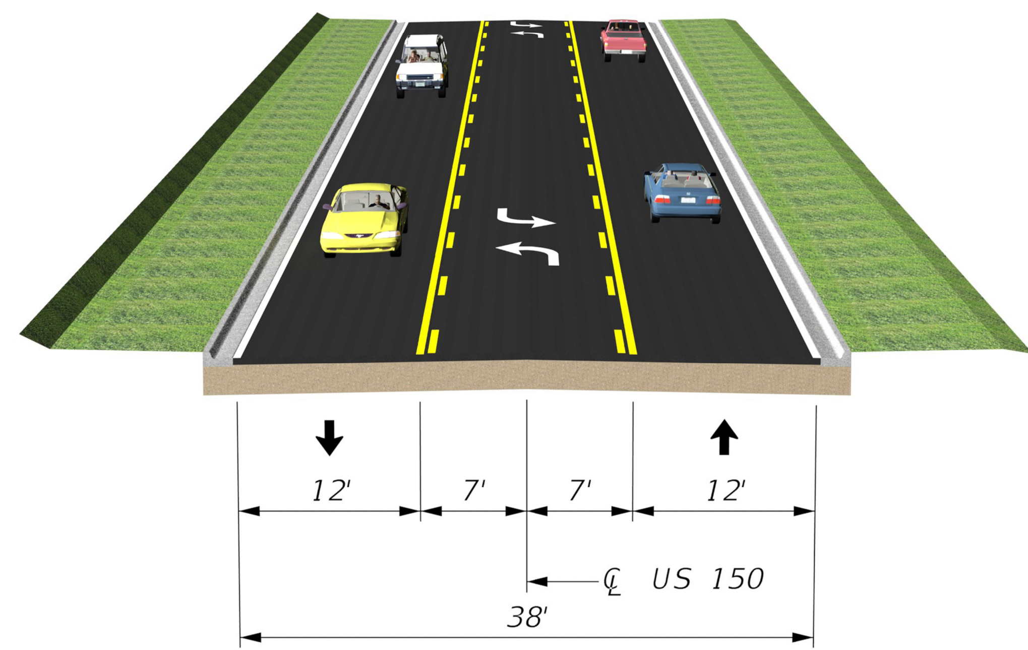
3-LANE URBAN TYPICAL SECTION
