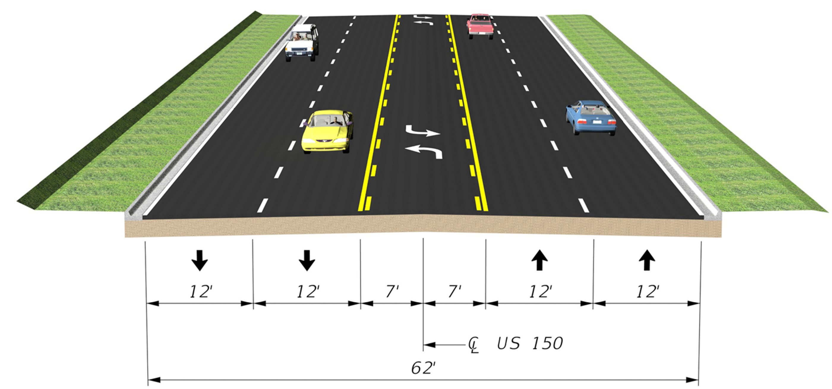
5-LANE URBAN TYPICAL SECTION
