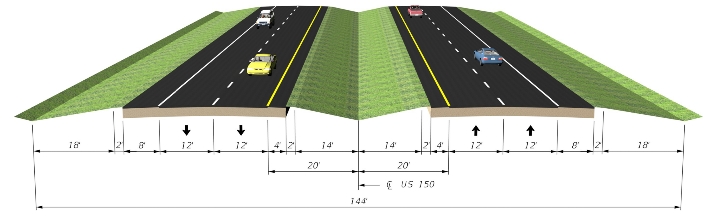
4-LANE DIVIDED RURAL TYPICAL SECTION
