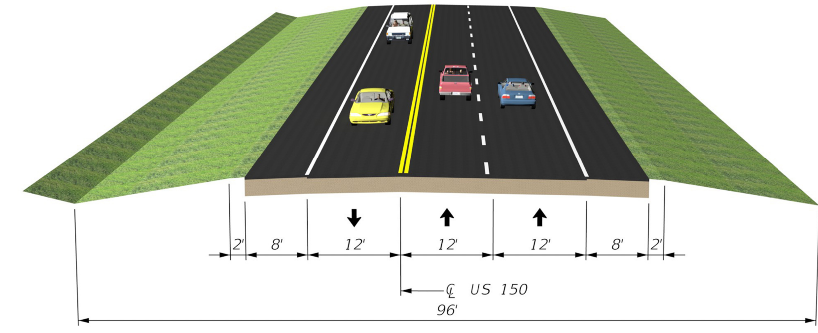
2-LANE PLUS PASSING LANE
