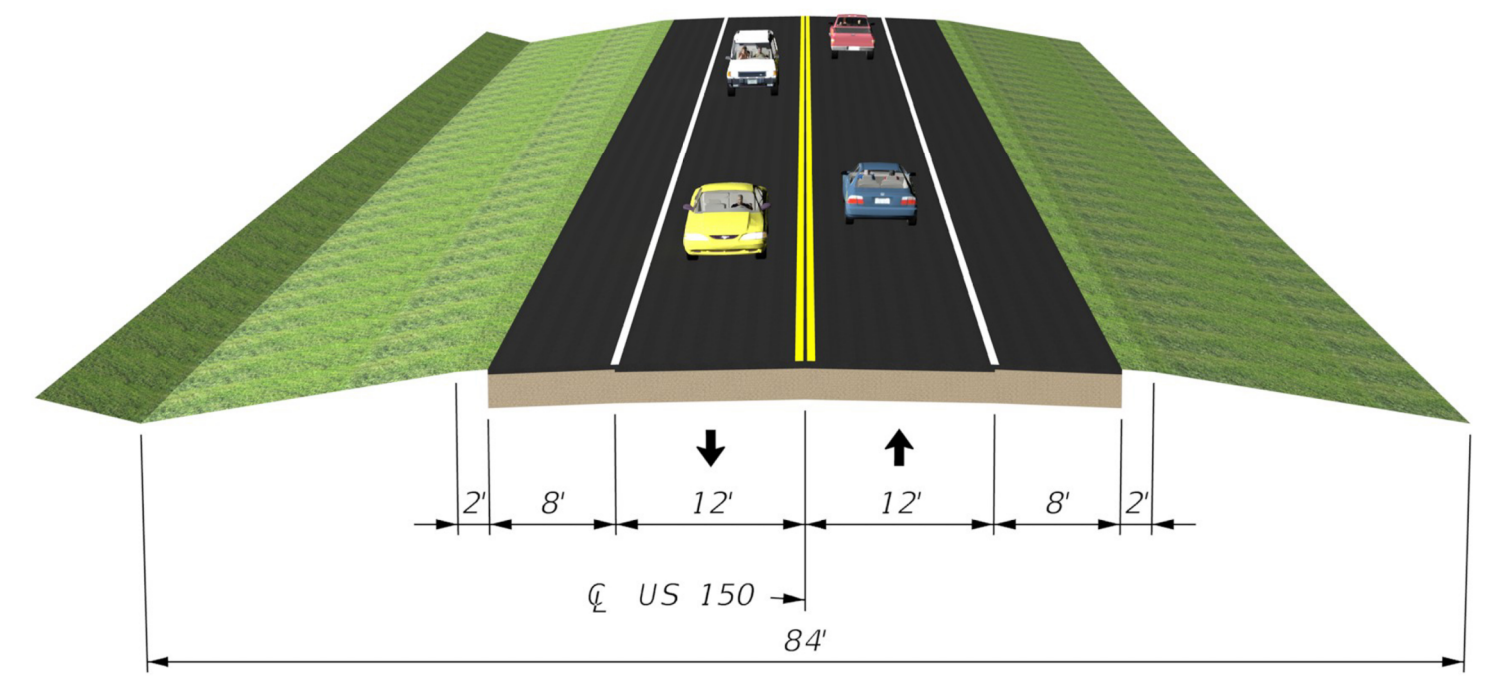
2-LANE RURAL TYPICAL SECTION
