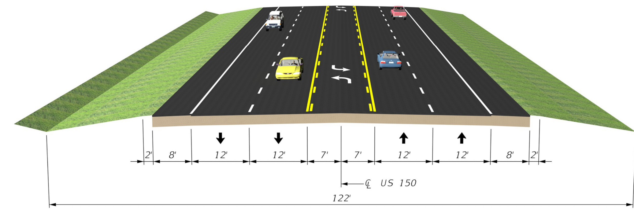
5-LANE RURAL TYPICAL SECTION
