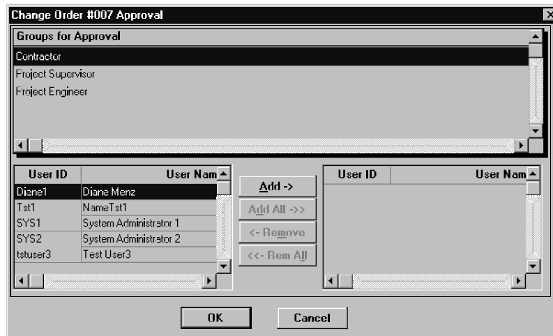
Figure 11-21. The Forward Change Order for Approval Window
