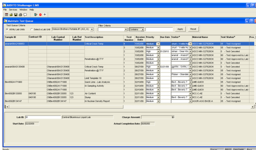
Figure 14-13. Maintain Test Queue Window
