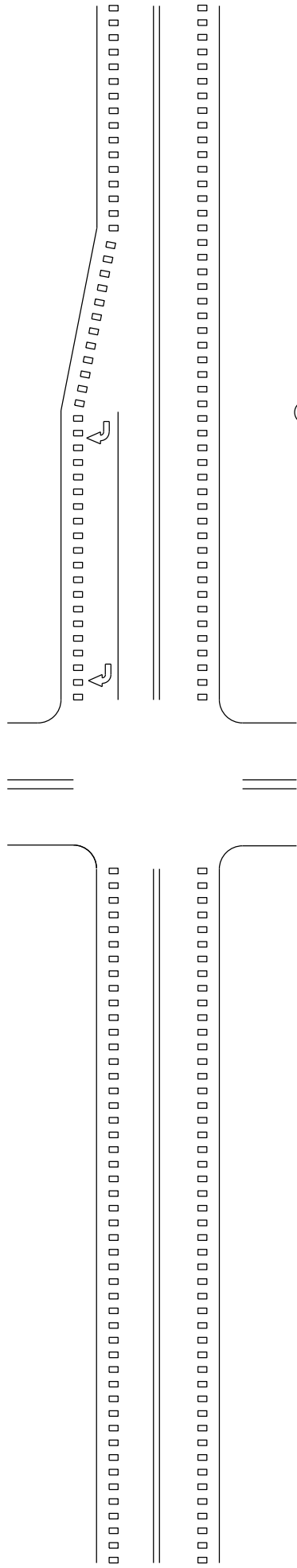
MAJOR INTERSECTIONS WITH OR WITHOUT RIGHT-TURN LANES
