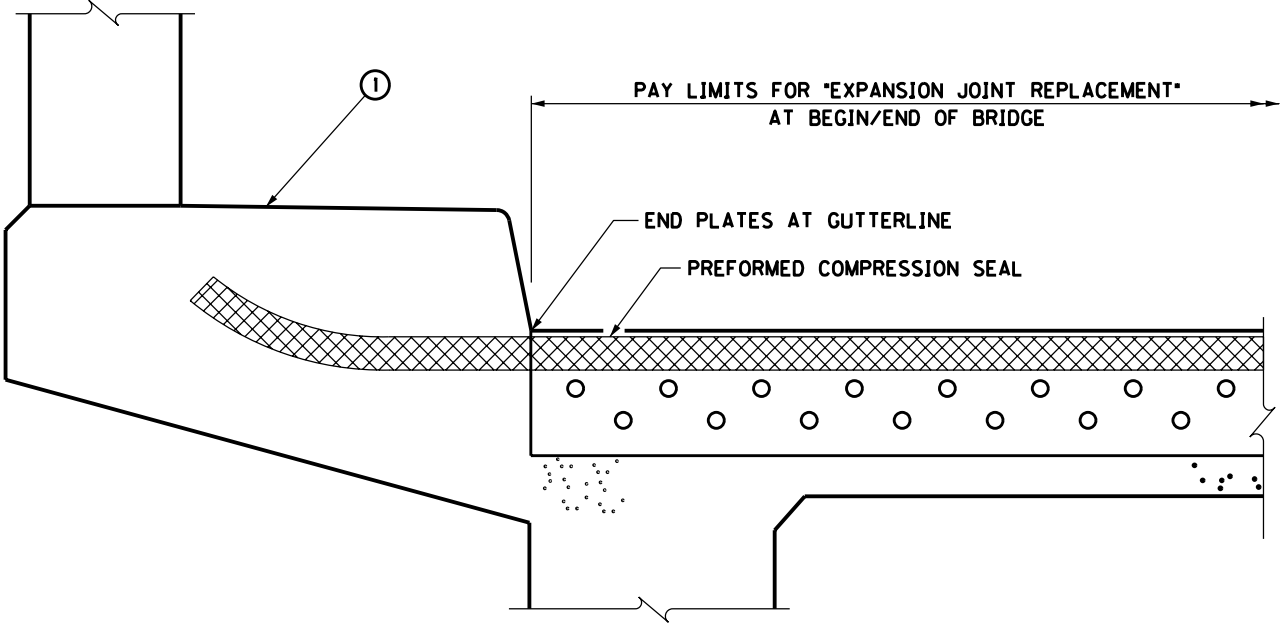
PROPOSED SECTION @ CURB
