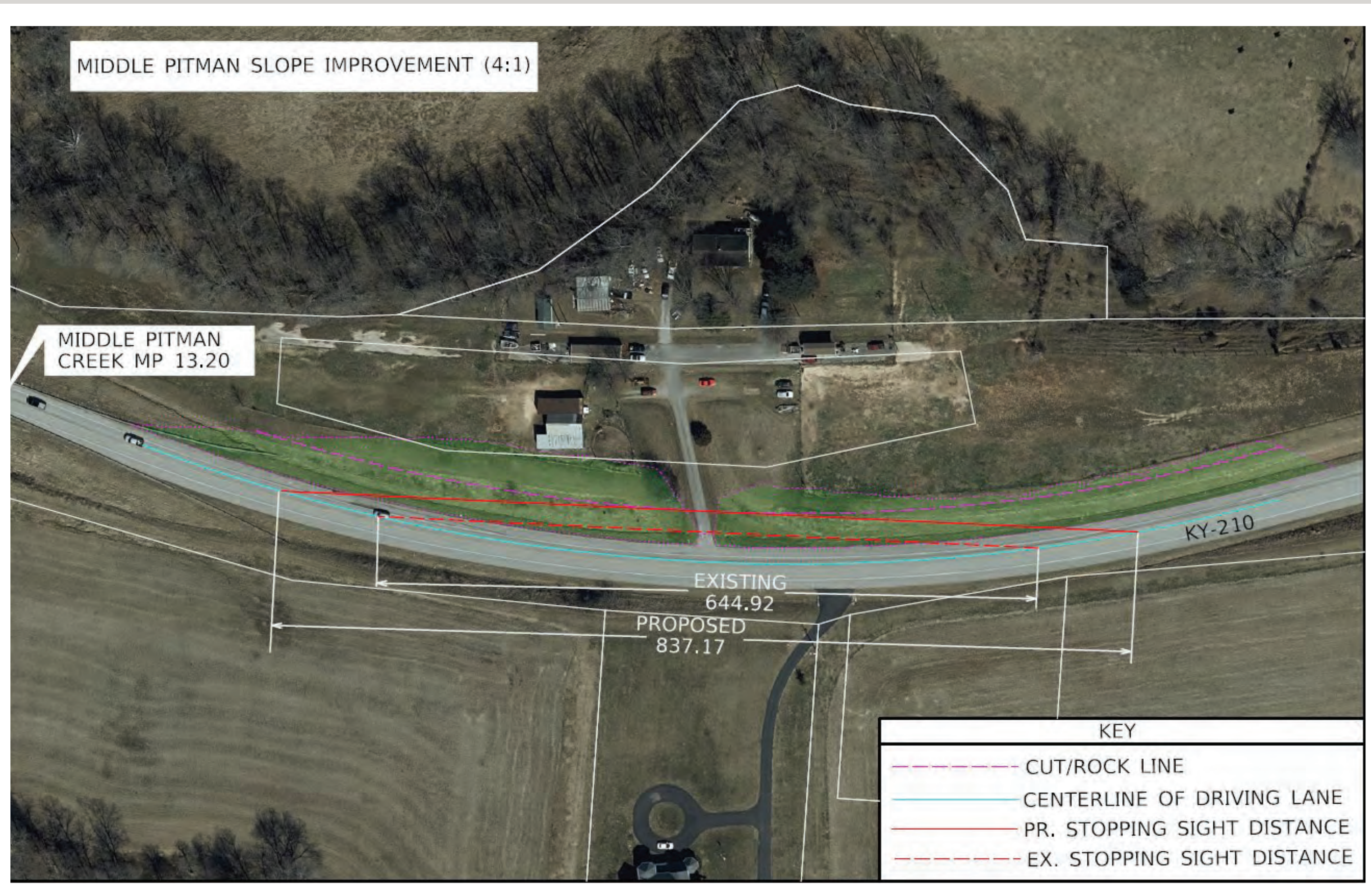
CUT BACK SLOPE.
