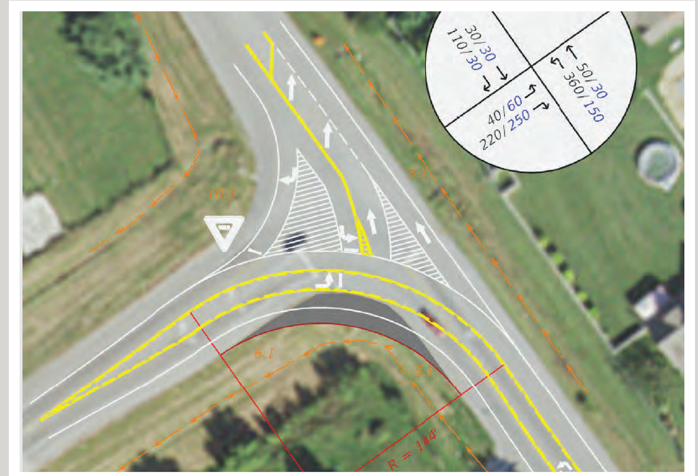
KY 1618 EASTBOUND FREE-FLOW CURVE.
